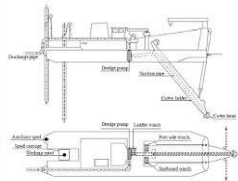
Cutter Suction Dredger (CSD)
